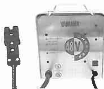
Automatic MAC 48-volt charger with MAC D.C. plug
